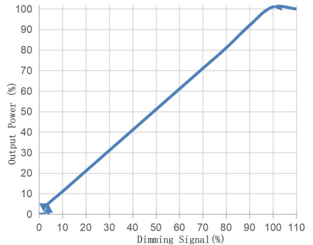
Fig 12. Output Power VS Dimming Signal
