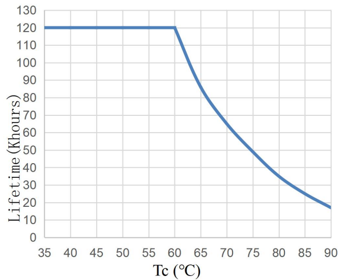
Fig 14. Lifetime VS Tc
