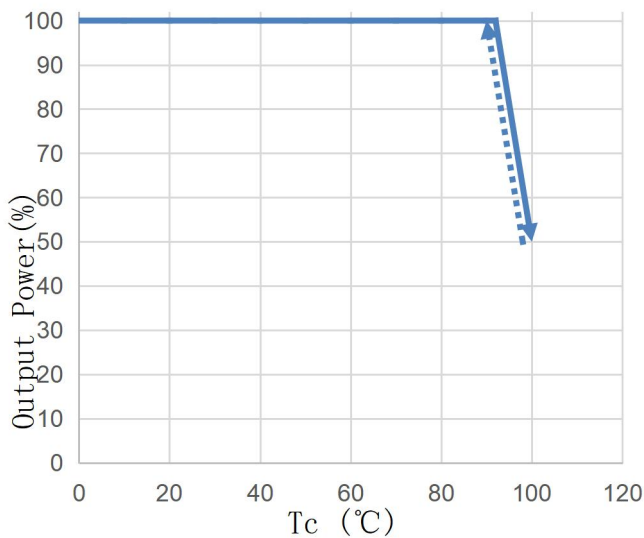
Fig 13. Output Power VS Tc
